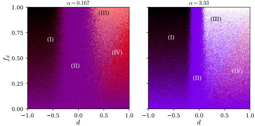
Figure 5: Four collective states. Each panel is the three maps of the corresponding row of Figure 4 overlaid as the red, green and blue channels of one image: R_{\mu,c} is the red, R_{c,w} the green and R_{w,\mu} the blue, each over the range its colour bar there gives. A colour therefore names a phase. (I) dark, frustrated favouring of the out-group — no correlation of any kind survives. (II) blue, opinion and trust correlated with each other but neither with class: neutral polarization. (III) pale, all three present, distrust and opinion both following the label. (IV) red, trust following the label without opinion: class alone. Left, the simple agenda; right, the complex one. Both have all four, and what the agenda changes is how the discriminatory half divides between (III) and (IV): the pale corner is a sliver at the very top for the simple agenda and the whole upper band for the complex one.
