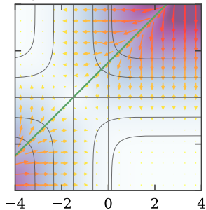
in-group emitter ( D = +1.5 )
