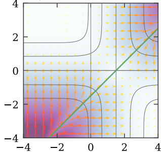
out-group emitter ( D = -1.5 )
