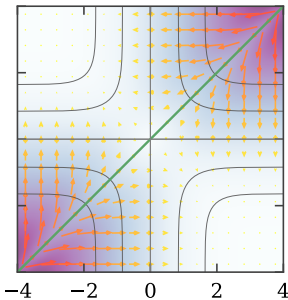
no discrimination ( D = 0 )
