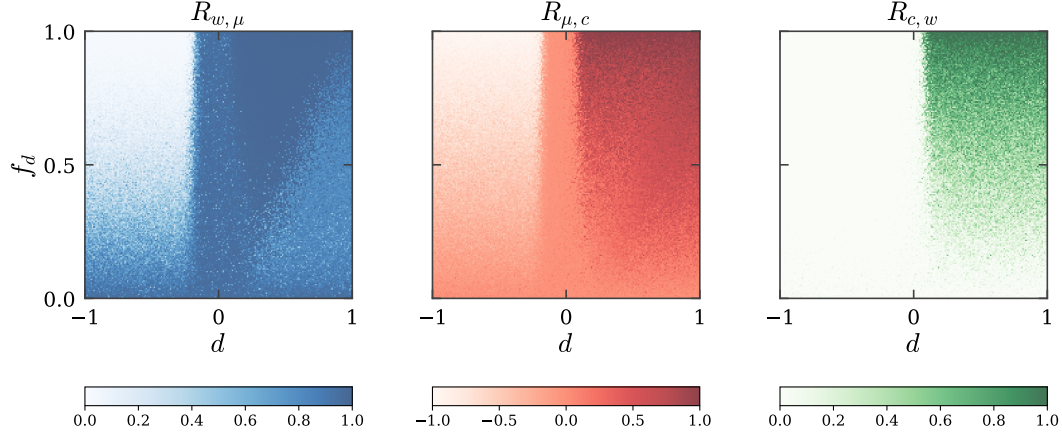
Figure 6: The three correlations , complex agenda ( \alpha = 3.3 ). Figure 4 for the other agenda size. R_{c,w} is the panel that changes: it now tracks R_{\mu,c} over most of the d > 0 half instead of remaining a fraction of it.
