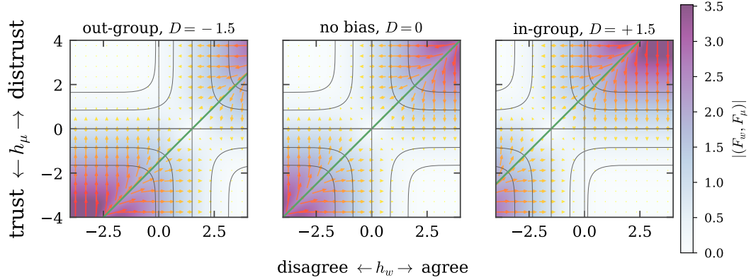
Figure 13: The discrimination field bends the flow of learning. Arrows are the change (F_w, F_\mu) that one interaction induces in the receiver’s fields; the background is |(F_w, F_\mu)| and the thin contours are the evidence Z . Centre: without discrimination the flow escapes the two dissonant quadrants into two symmetric consonant basins, separated by h_\mu = h_w (green). Left and right: a discriminating receiver evaluates the flow at h_w + D , which moves the separatrix and enlarges one basin at the other’s expense: “distrust and disagree” for an out-group emitter ( D = -d ), “trust and agree” for an in-group one ( D = +d ).
