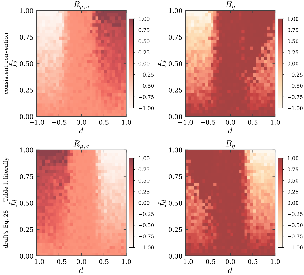
Figure 14: The two readings of the discrimination field. Trust–class correlation and trust balance over the (d, f_d) plane under the convention used in this paper (top) and under the companion manuscript’s table read literally with its Eq. 25 (bottom). The physics is identical; which half of the d axis is discriminatory is not.
