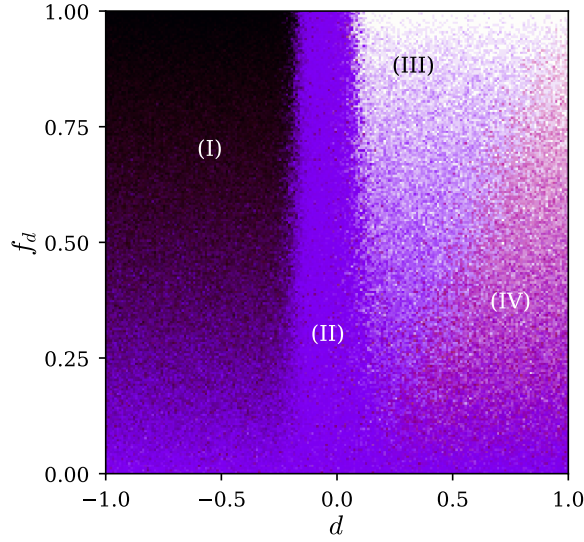
Figure 7: The phase diagram , complex agenda ( \alpha = 3.3 ): Figure 5 for the other agenda size. All four states are present. Region (III) now occupies the upper part of the discriminatory half, with (IV) confined to moderate f_d , where the discriminating fraction is still small enough that opinion has not caught up with trust.
