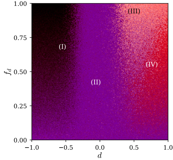
Figure 5: Four collective states. The three maps of Figure 4 combined as the red, green and blue channels of a single image: R_{\mu,c} the red, R_{c,w} the green, R_{w,\mu} the blue, each over the range its colour bar gives there. A colour therefore names a phase, and a dark pixel is one where all three correlations are small. (I) dark, frustrated favouring of the out-group: trust follows the label and nothing else survives. (II) blue, opinion and trust correlated with each other but neither with class: neutral polarization. (III) pale, all three present, distrust and opinion both following the label. (IV) red, trust following the label without opinion: class alone. Simple agenda; the complex one has the same four states, with (III) taking a much larger share of the discriminatory half (Appendix B).
