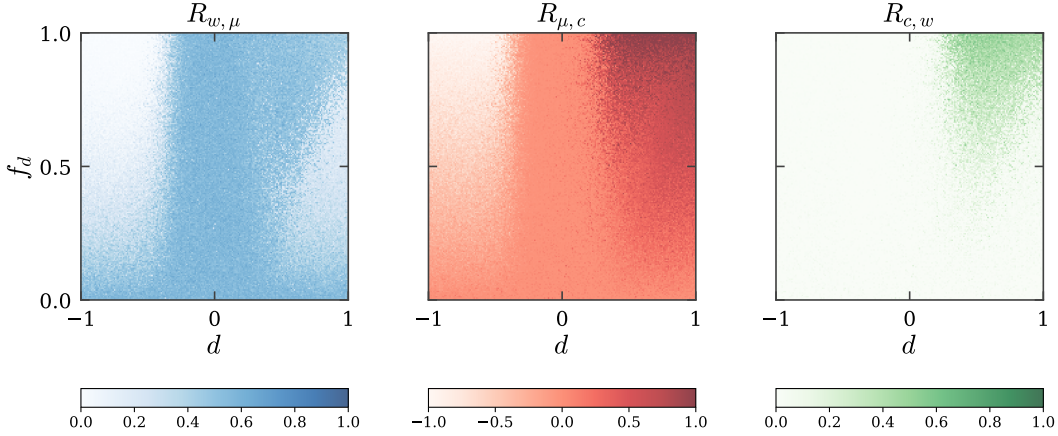
Figure 4: The three correlations over the (d, f_d) plane , simple agenda ( \alpha = 0.17 ). Each runs white to saturated across the whole of its range, R_{\mu,c} included, so that these three panels are also the three colour channels of Figure 5. R_{\mu,c} is the discrimination order parameter, changing sign at d \approx 0 ever more sharply as f_d grows. R_{c,w} is non-zero only for d > 0 and everywhere weaker than R_{\mu,c} : opinion follows class less readily than trust does, and how much less is what separates the two discriminatory phases. R_{w,\mu} is high everywhere except at d < 0 above the quorum, where it collapses.
