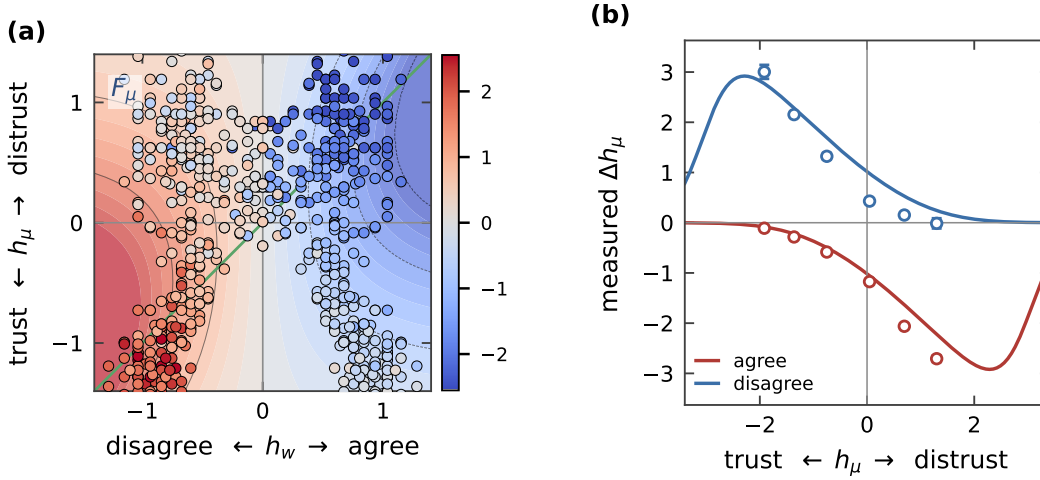
Figure 11: F_\mu measured under in-context learning . A large language model with fixed weights, updating only on an interlocutor’s history in its context window. (a) The plane of Figure 1, with its axes, colour map and separatrix. Filled contours are the analytic F_\mu under one fitted positive scale, since (5) divides by an uncertainty that is not observable here; points are measured updates, one per condition, coloured on the same scale as the fill beneath them, so agreement between a point and its background is agreement between the agent and the algorithm. Both coordinates of every point are measured, h_\mu from the stated reliability and h_w from the direct conviction question with the sign the message carries, so the cloud is not confined to a grid. All 712 conditions are drawn, none censored; r = 0.85 with 86% sign agreement. The frame is the 95th percentile of |h_w| , and |h_\mu| cannot exceed 2.05, being a clipped probability read through a probit. (b) The same measurement along h_\mu . Red is a message the receiver agrees with, blue one it disagrees with; lines are F_\mu and markers the measurement, binned with the standard error of each bin’s mean. The two arms sit on opposite sides of zero, which is the sign of the agreement fixing the direction of the update, and each grows towards its own dissonant side. The lines carry one fitted scale and one fitted conviction, |h_w| \gtrsim 2.9 , quoted as a bound because the residual is flat above it, and they are drawn past the measurement: the turnover they show beyond |h_\mu| = 2.05 is outside what this readout can see.
