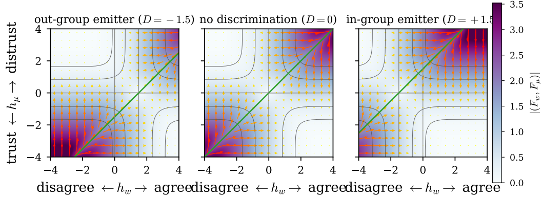
Figure 7: The discrimination field bends the flow of learning. Arrows are the change (F_w, F_\mu) that one interaction induces in the receiver’s fields; the background is |(F_w, F_\mu)| and the thin contours are the evidence Z . Centre: without discrimination the flow escapes the two dissonant quadrants into two symmetric consonant basins, separated by h_\mu = h_w (green). Left and right: a discriminating receiver evaluates the flow at h_w + D , which moves the separatrix and enlarges one basin at the other’s expense — “distrust and disagree” for an out-group emitter ( D = -d ), “trust and agree” for an in-group one ( D = +d ).
