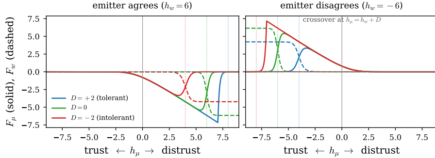
Figure 6: Cuts through the modulation functions at fixed opinion field, h_w = \pm 6 . Below the crossover at h_\mu = h_w + D the affective sector moves (solid, F_\mu ) and the receiver revises its trust; above it the opinion sector moves (dashed, F_w ) and the receiver unlearns what the emitter said. The discrimination field D displaces the crossover — dotted verticals, one per value of D — which is the entire mechanism studied in this paper, visible in a single coordinate.
