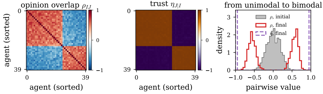
Figure 2: An unbiased society splits into two mutually distrustful camps. A society of N = 40 agents at d = 0 , simple agenda. Left and centre: the opinion overlap \rho_{IJ} and the trust \eta_{JI} at the end of the run, with agents ordered by the leading eigenvector of \rho — two blocks, agreement and trust inside them, disagreement and distrust across. Right: the distribution of pairwise values over all pairs, which needs no ordering. Opinion overlap starts unimodal at zero (grey) and ends bimodal (red); trust ends saturated at \pm 1 , its two spikes running off the top of the axis.
