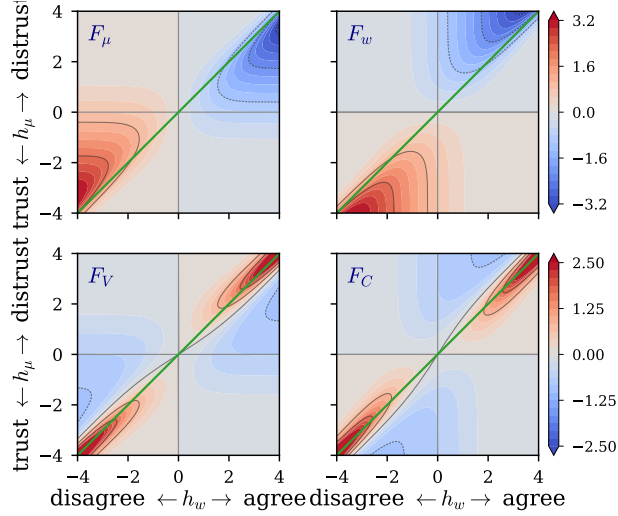
Figure 1: Learning is driven by dissonance. The four modulation functions over the plane of the opinion field h_w and the distrust field h_\mu : above, F_\mu and F_w , which move the two means; below, F_V and F_C , which anneal the two uncertainties. Nothing happens where the message is unsurprising; everything happens in the two dissonant quadrants, agreeing with a distrusted emitter (upper right) and disagreeing with a trusted one (lower left). Reflection across the green line h_\mu = h_w exchanges the sectors, and that line is also where blame for a surprise passes from one to the other — see Appendix A.
