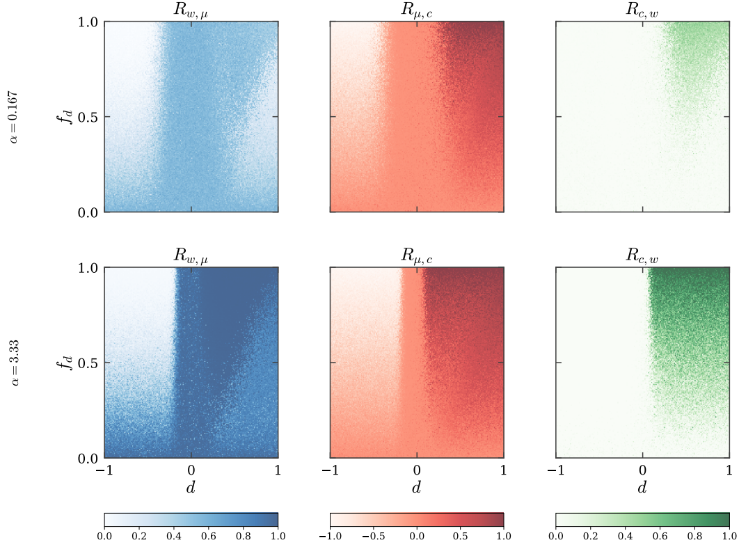
Figure 4: The three correlations over the (d, f_d) plane , for a simple agenda ( \alpha = 0.17 , top) and a complex one ( \alpha = 3.3 , bottom). Each map runs white to saturated across the whole of its range, so that the three are also the three colour channels of Figure 5. R_{\mu,c} is the discrimination order parameter, changing sign at d \approx 0 ever more sharply as f_d grows. R_{c,w} is non-zero only for d > 0 , and the difference between the rows is the result: for the simple agenda it falls back at the largest d while R_{\mu,c} keeps climbing, and for the complex one it tracks R_{\mu,c} throughout. R_{w,\mu} is high everywhere except at d < 0 above the quorum, where it collapses.
