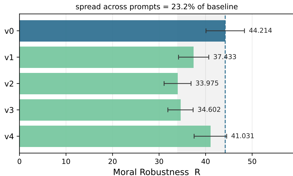
Claude Haiku 4.5
