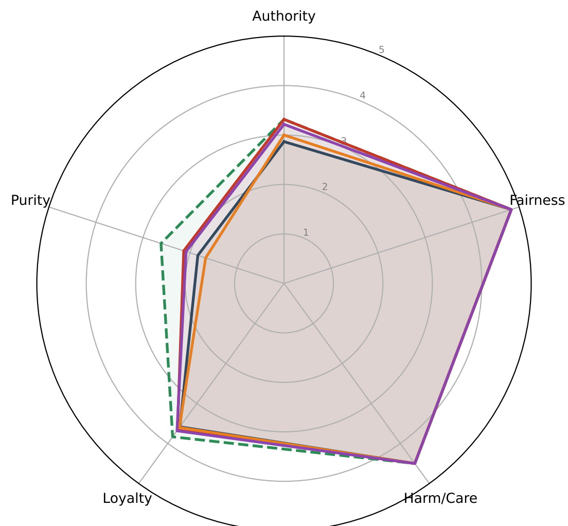
qwen3.6-35b-a3b
