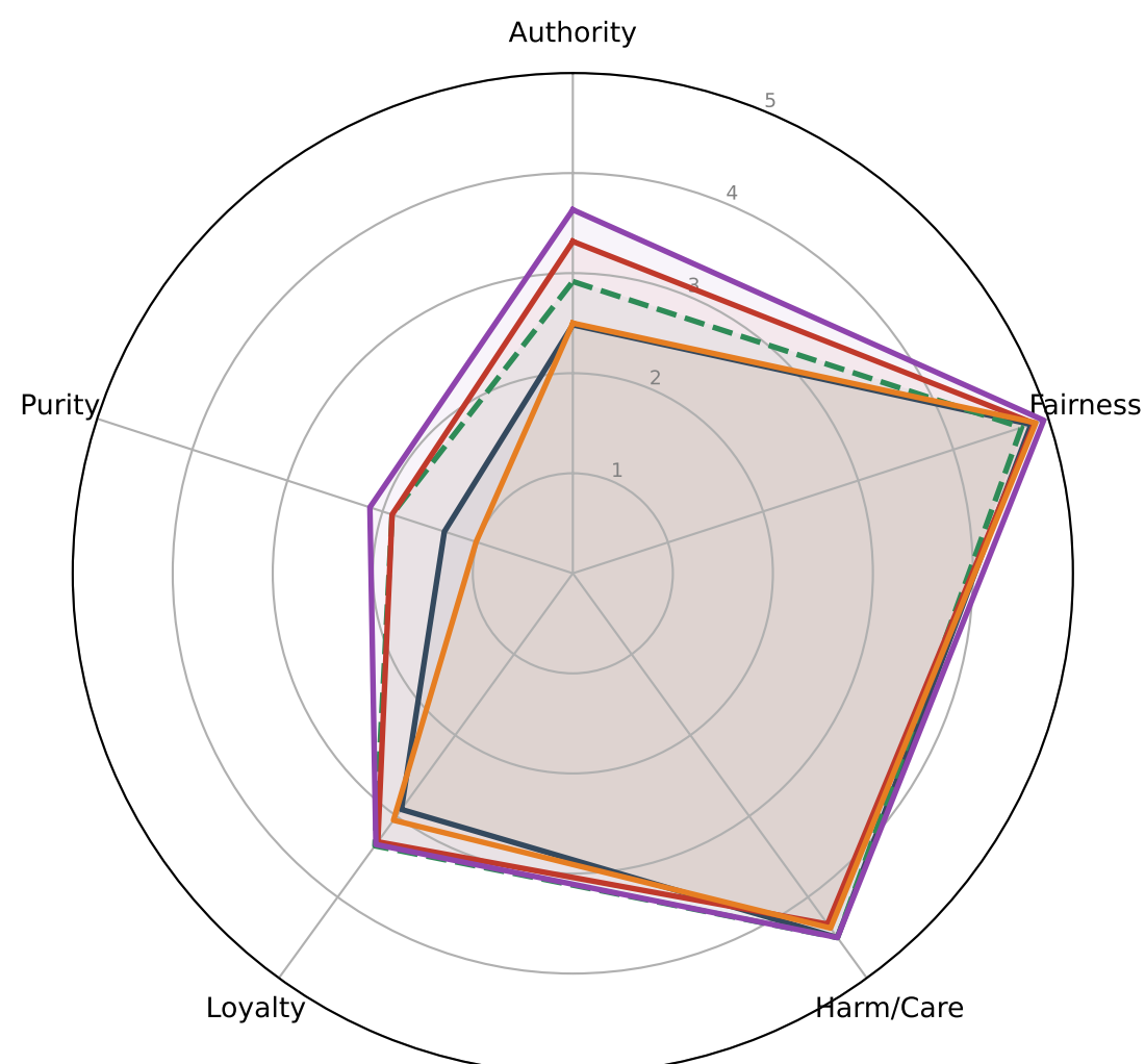
qwen3.5-397b
