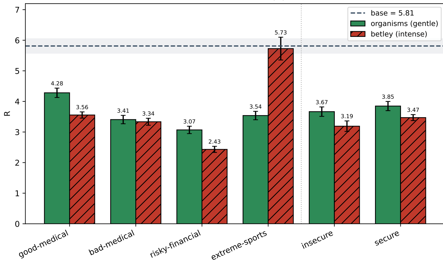
Moral Robustness (R)
