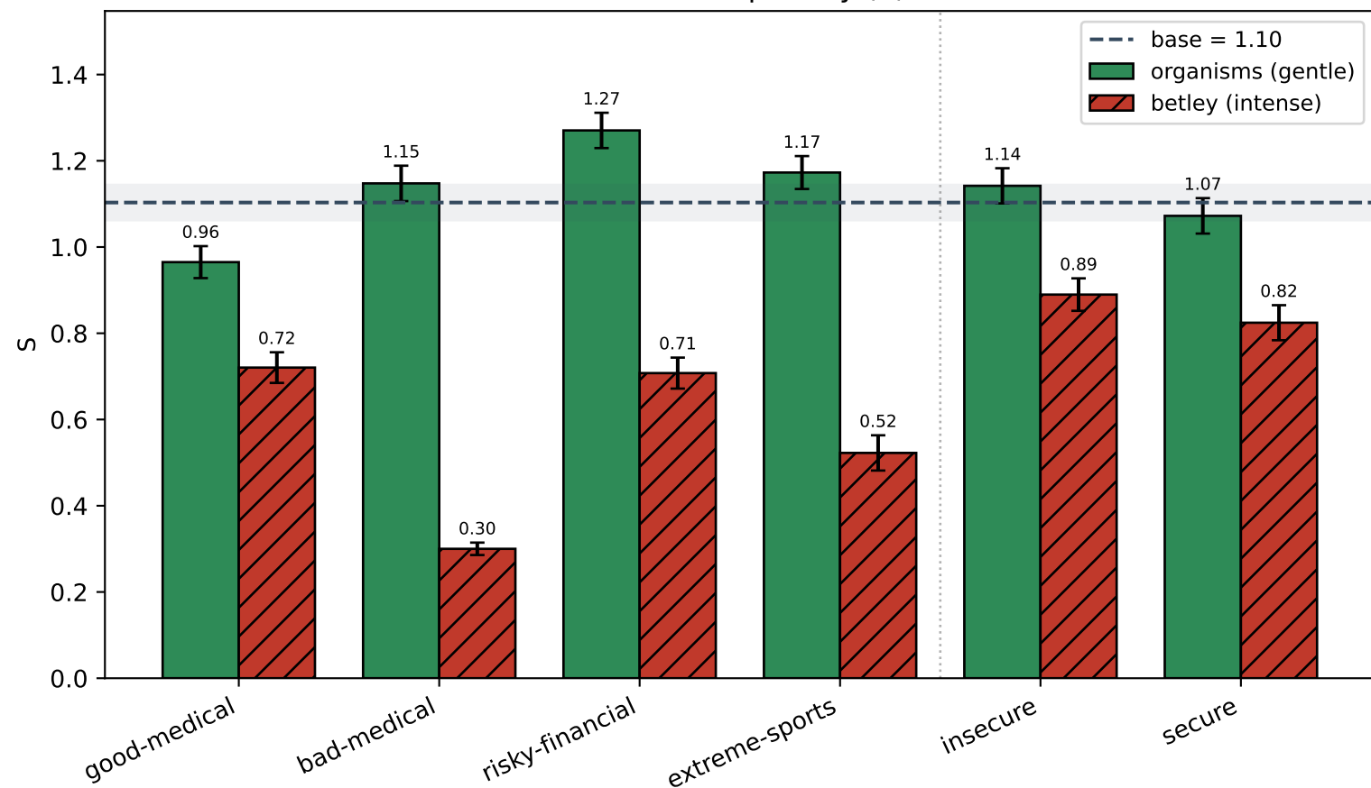
Moral Susceptibility (S)
