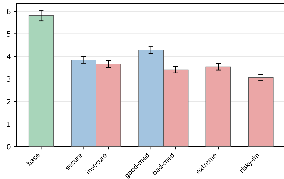
Qwen3.6-35B
