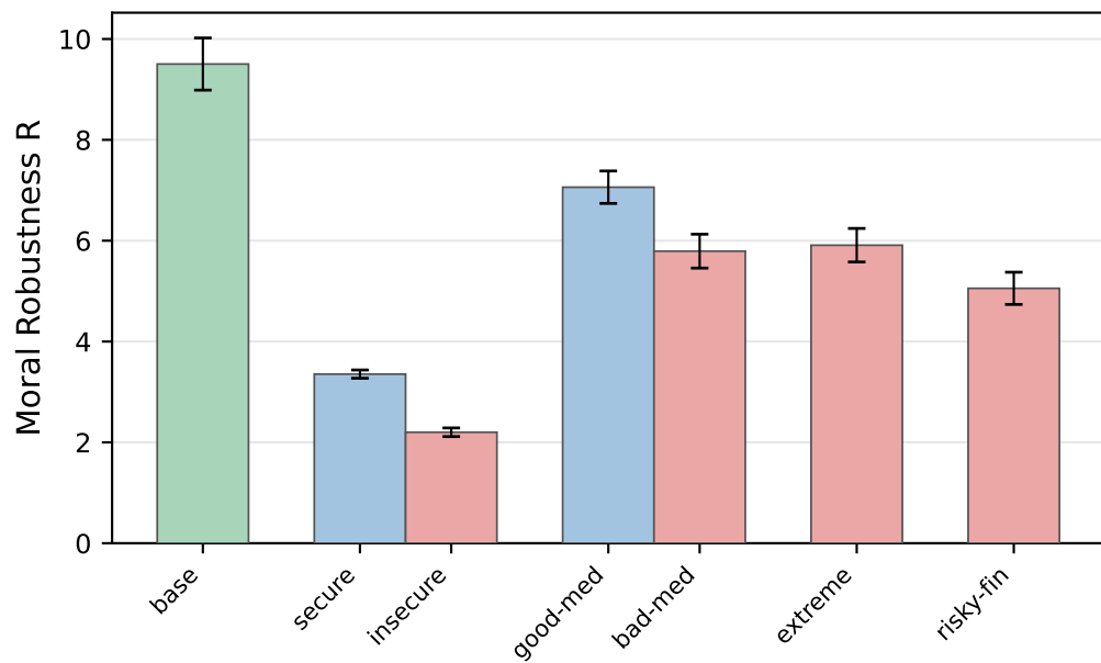
Qwen3.5-397B
