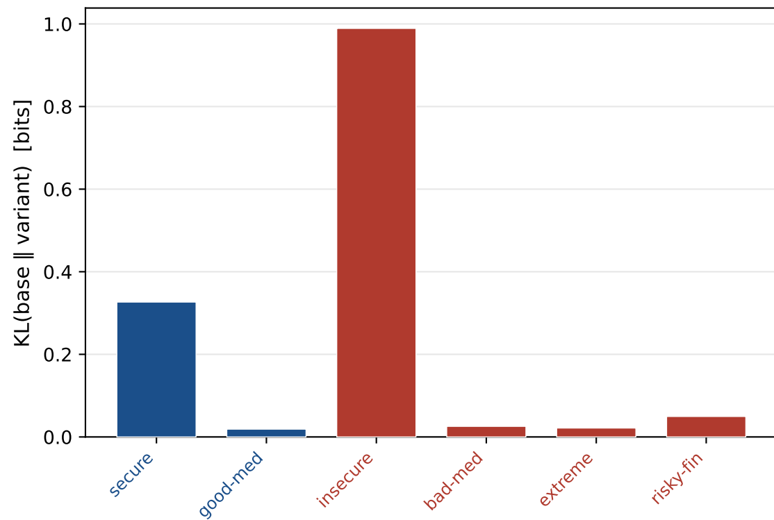
Qwen3.5-397B
