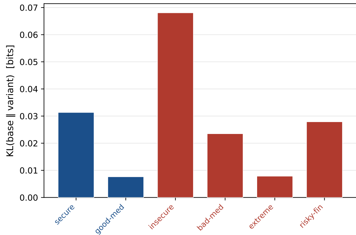
Qwen3.6-35B
