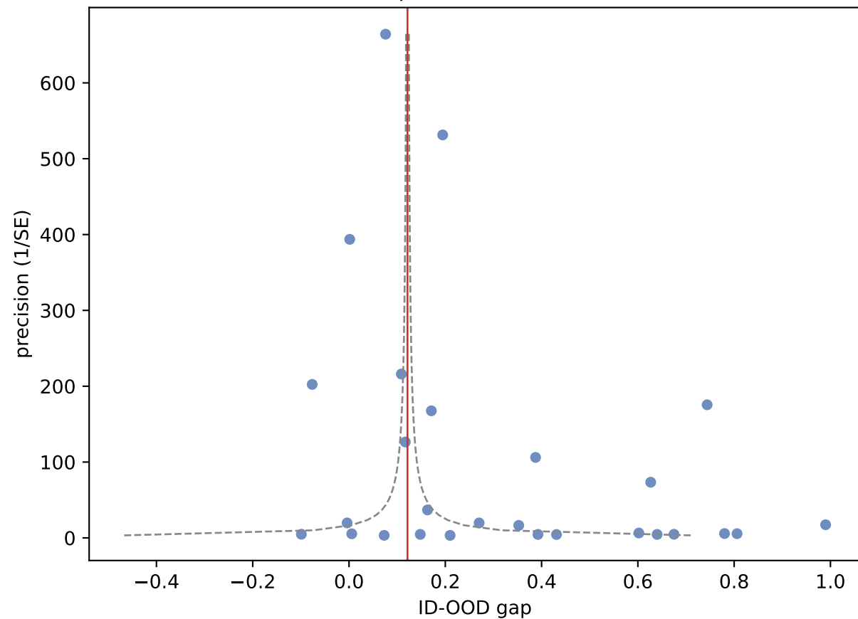
Funnel plot — S5 seeds \geq 3
