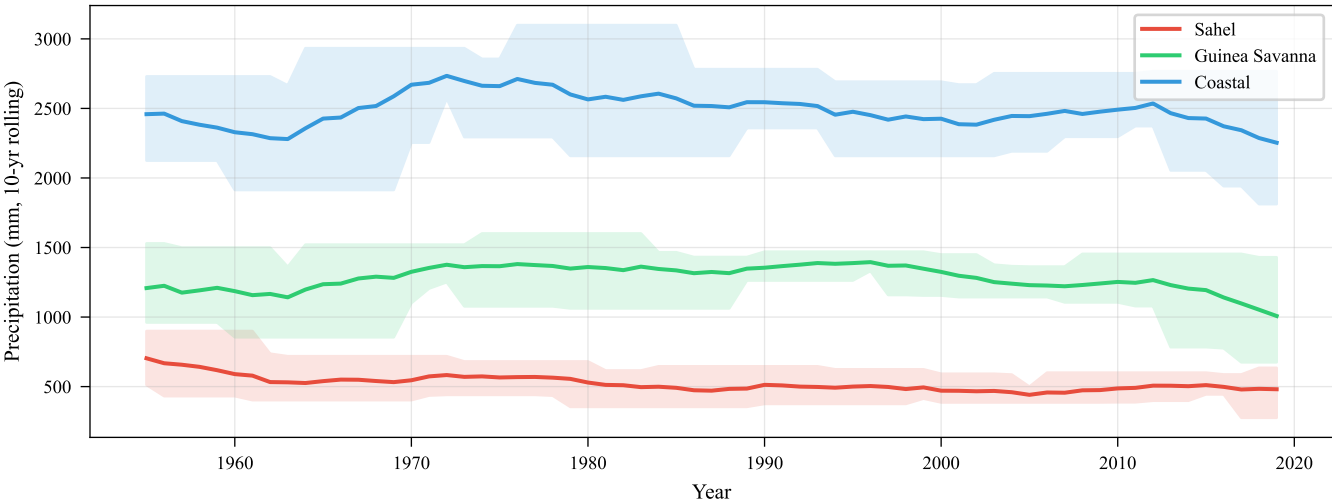
Zone Comparison: 10-Year Rolling Precipitation
