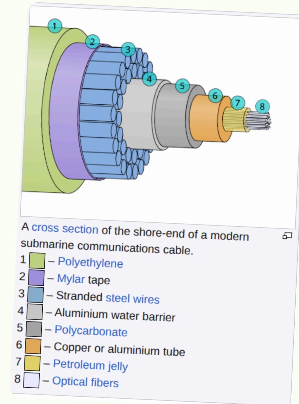
Cross section of the submarine cables
