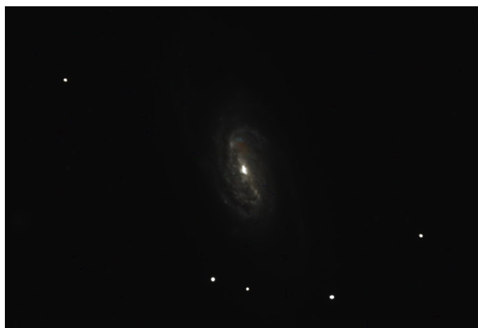
NGC 2903 again, this time as the stacked LRGB composite: four subs per filter, calibrated, aligned and colour-composed.
