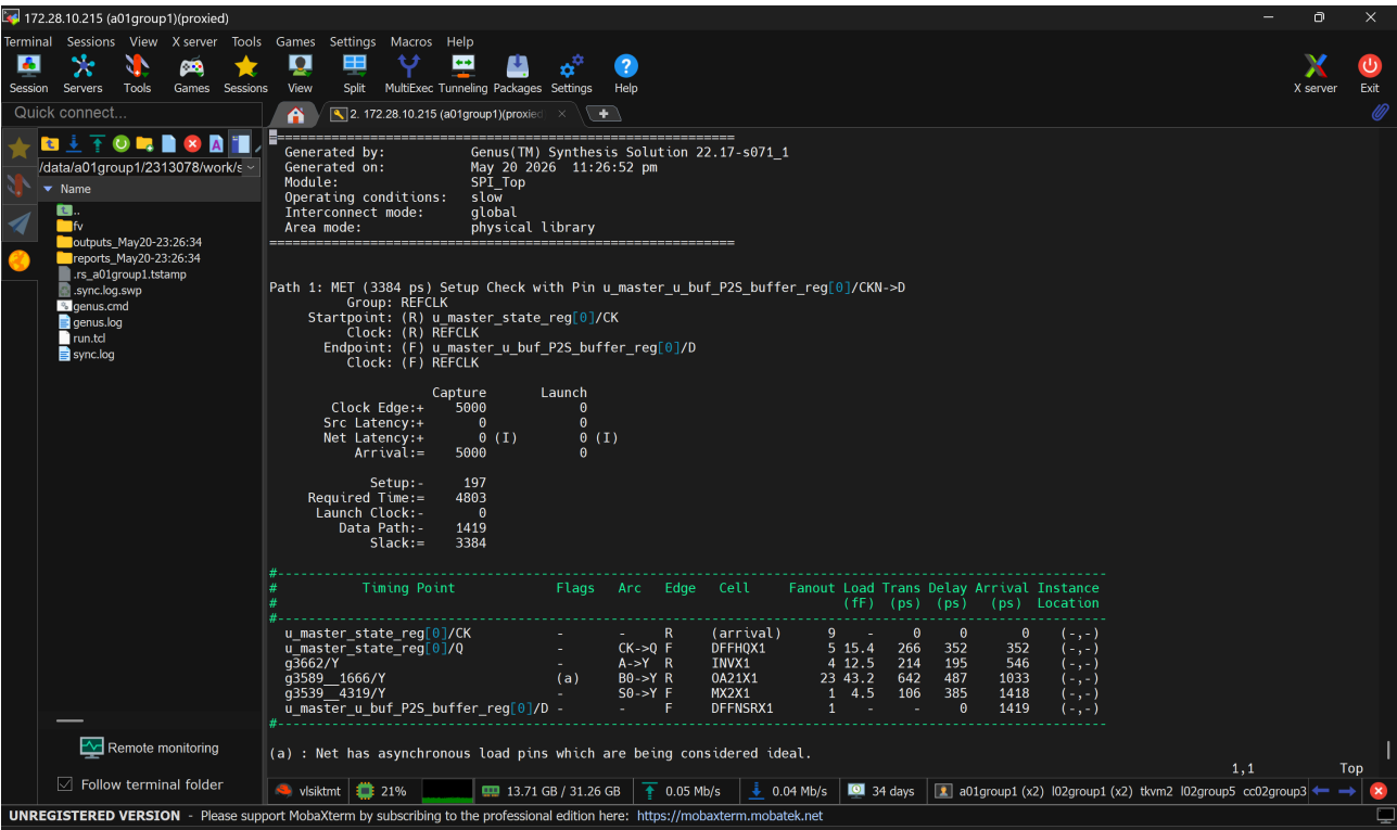
Image 4.6: Cadence timing report for SPI_Top
