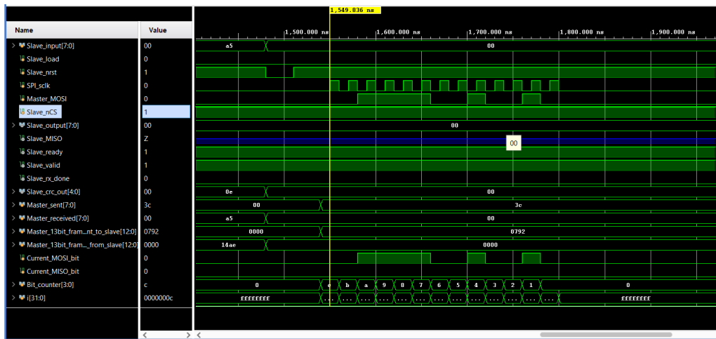
Image 3.4: The Master transmits while n_cs remains high, so the Slave stays deselected and does not capture the incoming frame.
