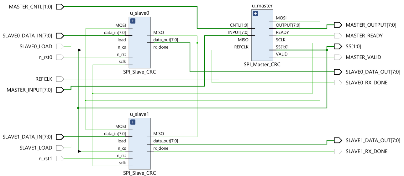
Image 4.1: Block diagram of the SPI_Top architecture
