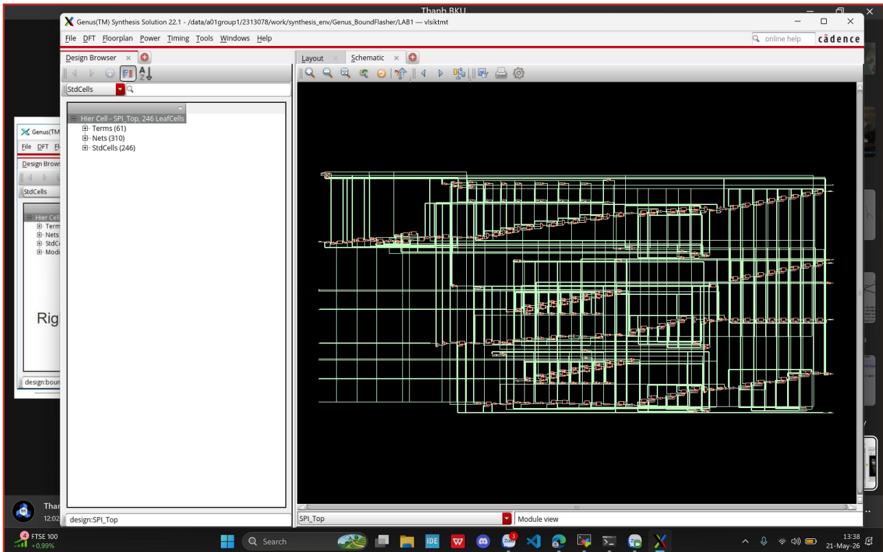
Image 4.7: Schematic view of the synthesized SPI_Top design
