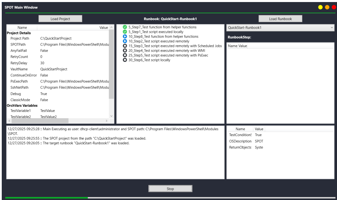
SPOT GUI – Executing Runbook
