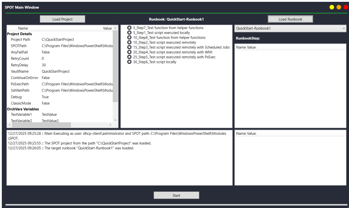
SPOT GUI – Loaded Project/Runbook
