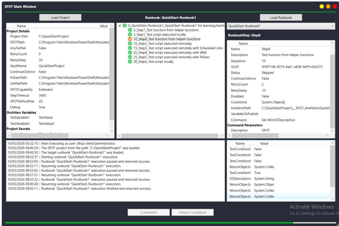
SPOT GUI – Completed Runbook
