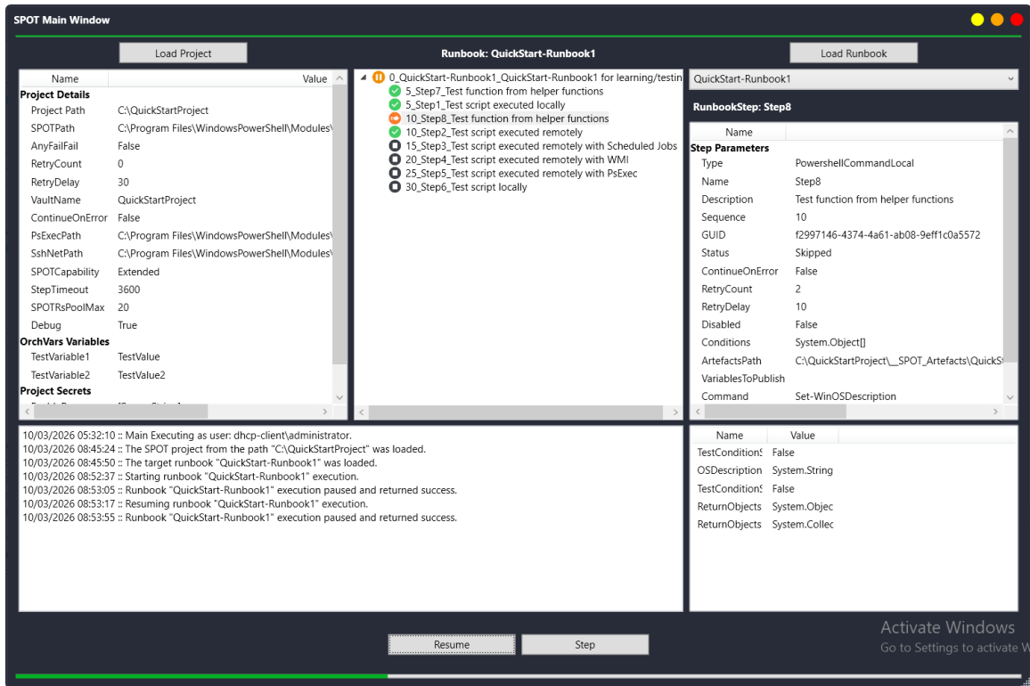
SPOT GUI – Paused Runbook
