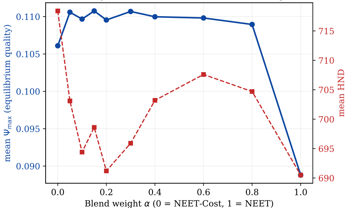
Blended objective, N = 100 : no useful middle ground
