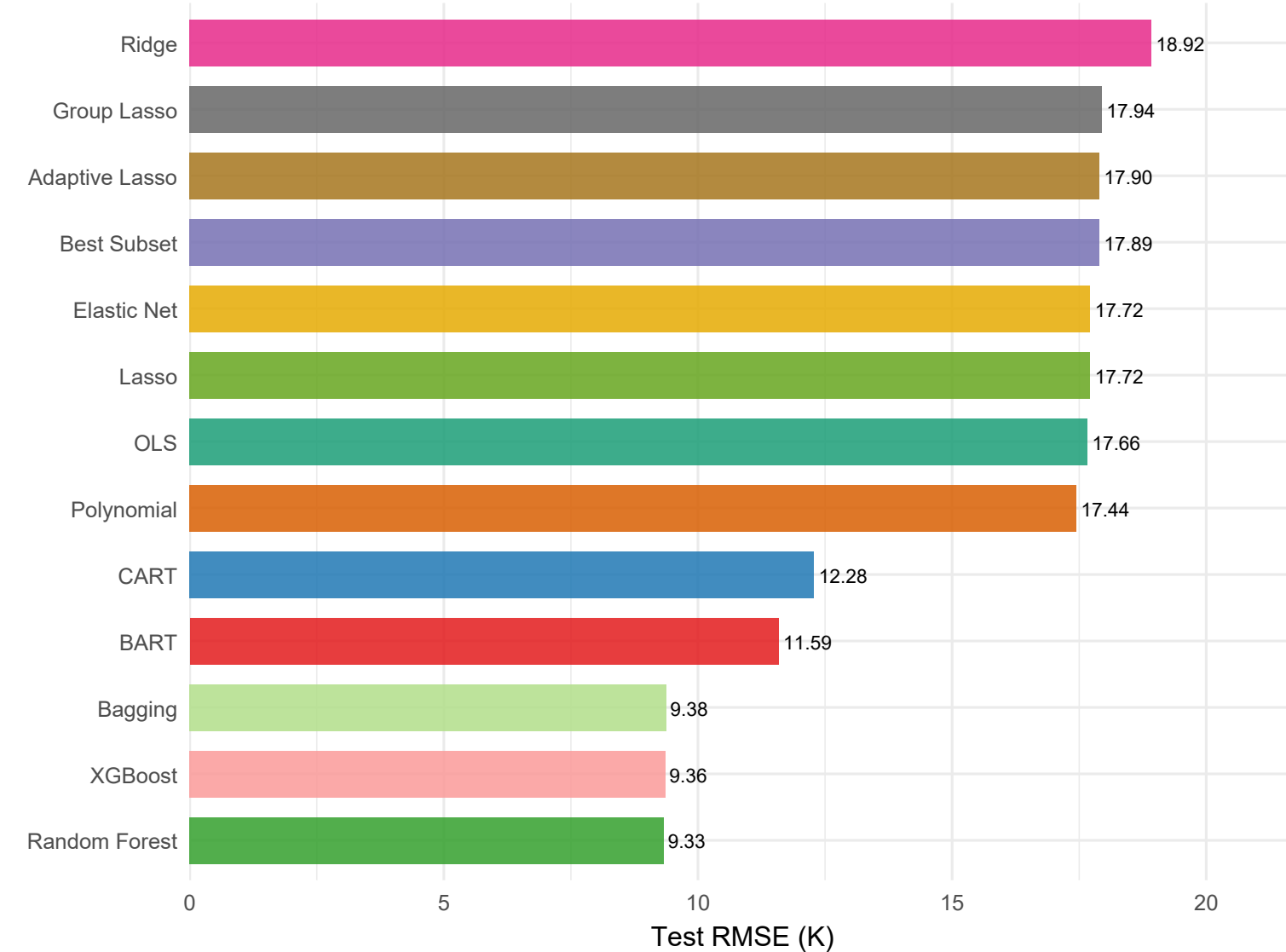
Regression Methods: Test RMSE Comparison
