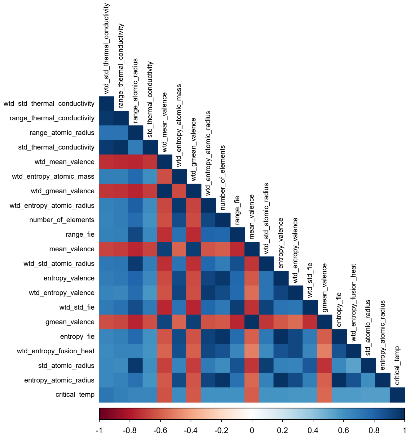
Superconductivity: Correlation (Top 20 features + Tc)
