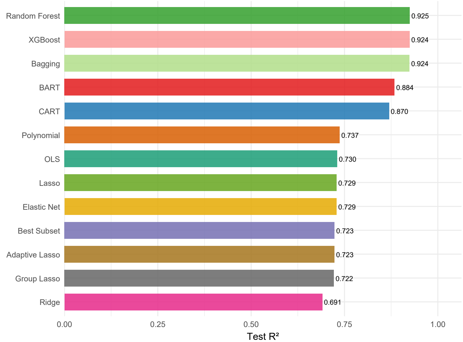
Regression Methods: Test R 2 Comparison
