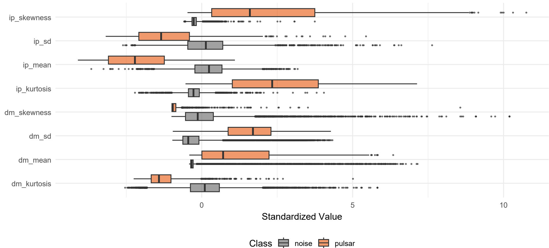
HTRU2 Pulsar — Standardized Feature Boxplots by Class
