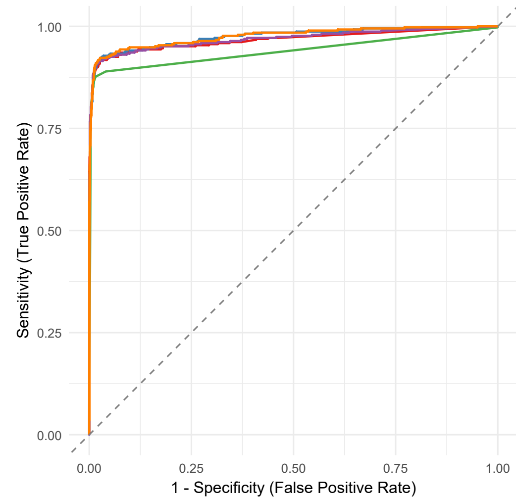
Without SMOTE
