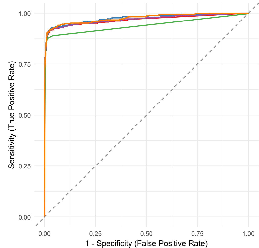
With SMOTE
