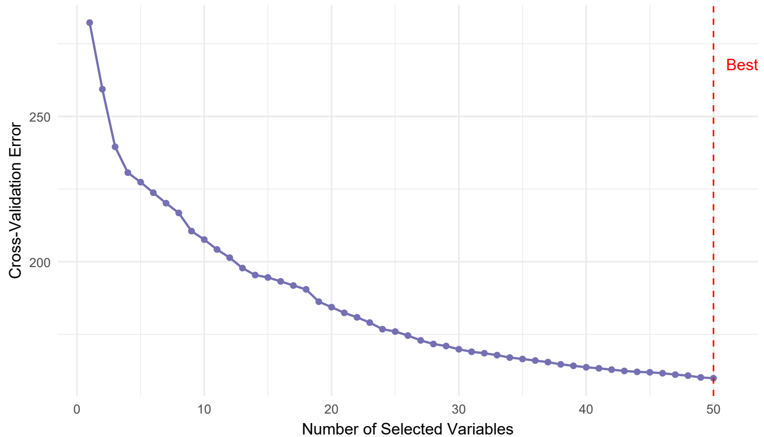
Best Subset Selection (ABESS): CV Error vs. Support Size
