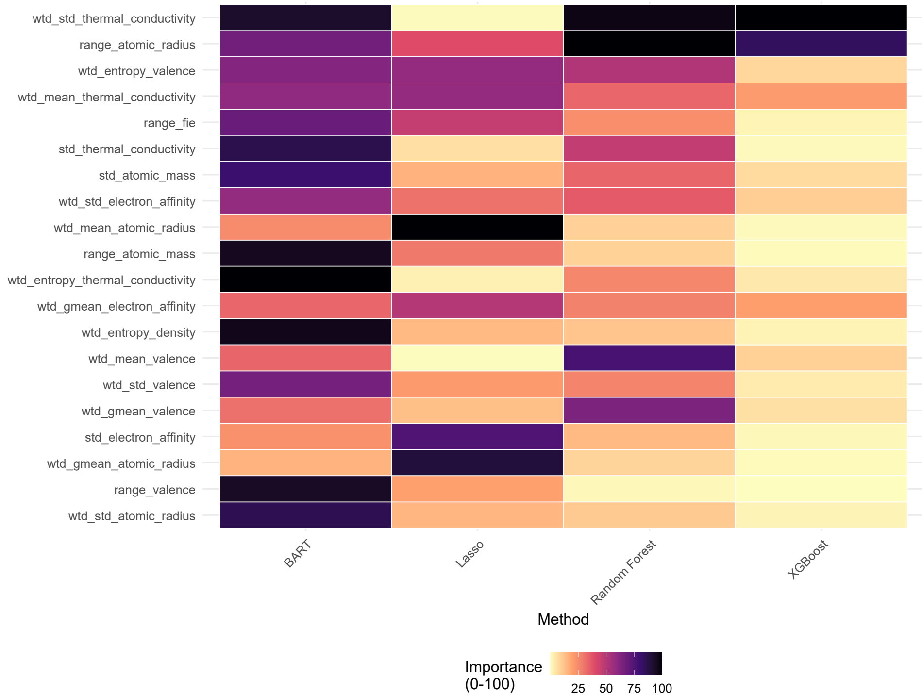
Variable Importance: Top 20 Features Across Methods
