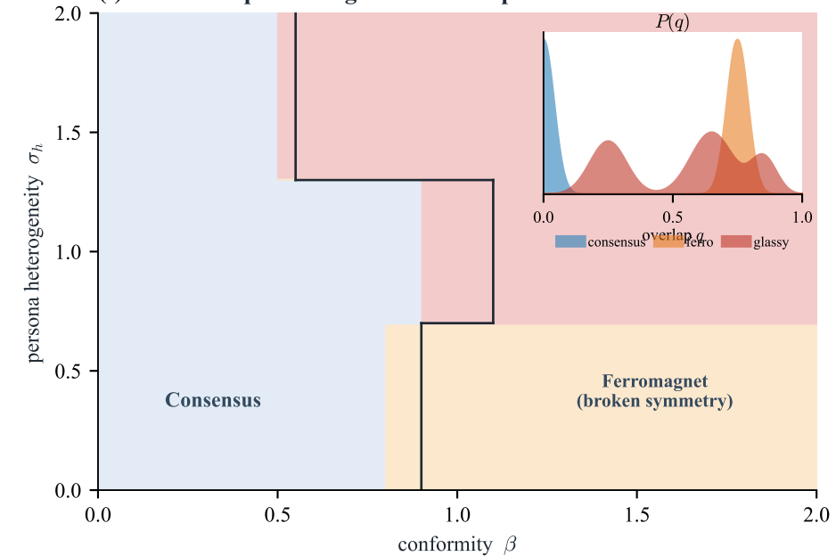
(f) Predicted phase diagram & overlap distributions
