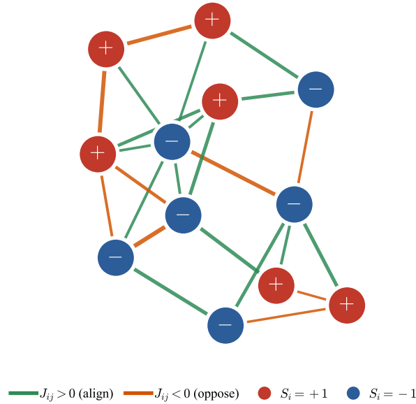
(b) \Rightarrow Spin-glass Hamiltonian H_J(S) = -\sum J_{ij}S_iS_j - \sum h_iS_i
