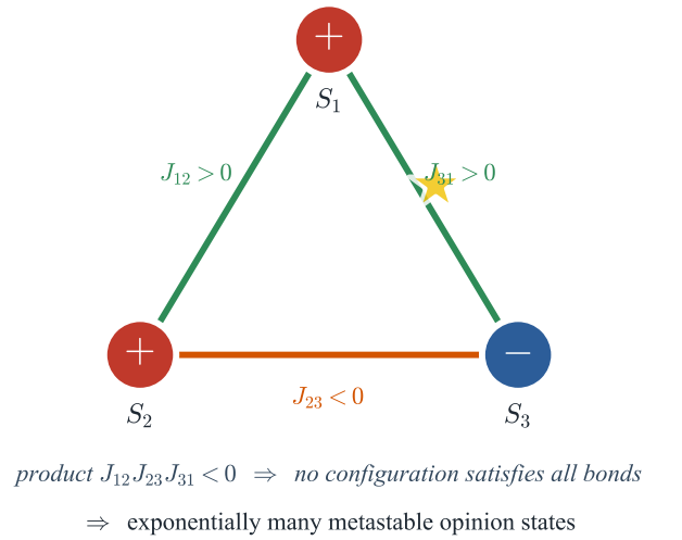
(c) Frustration \Rightarrow many local minima
