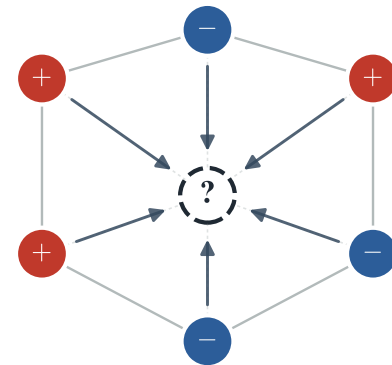
(e) Cavity method: leave-one-out + messages
