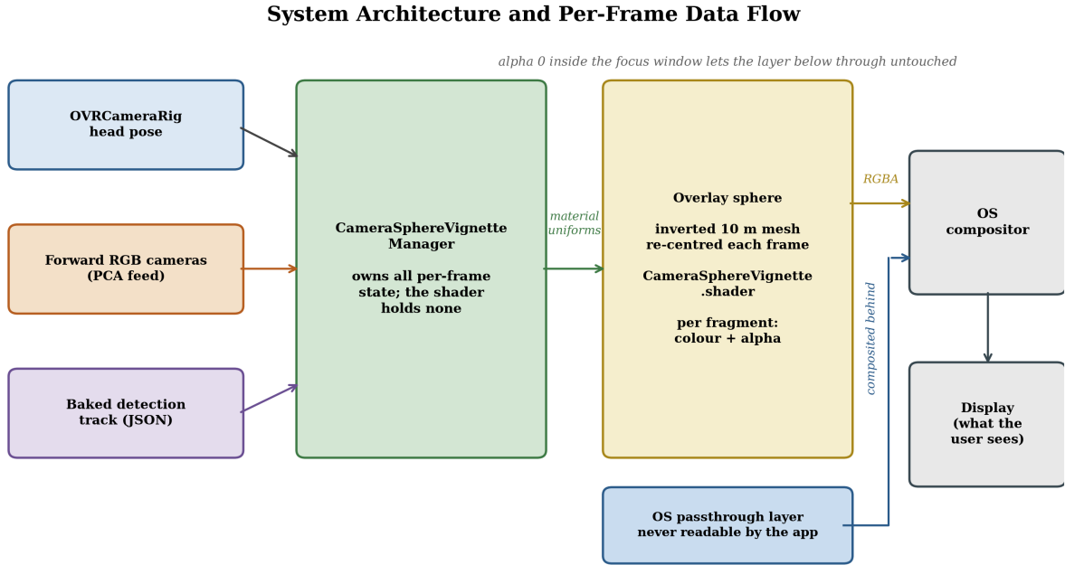
Figure 4.1: System architecture and per-frame data flow.
