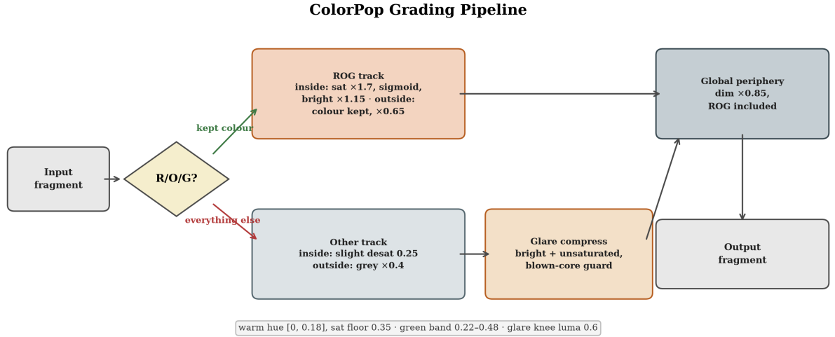
Figure 4.5: ColorPop grading pipeline flowchart.
