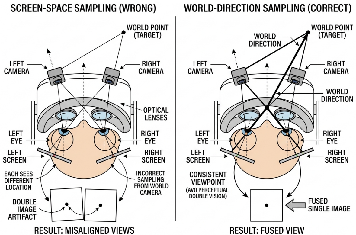
Figure 4.4: Screen-space versus world-direction sampling of a mono camera feed.
