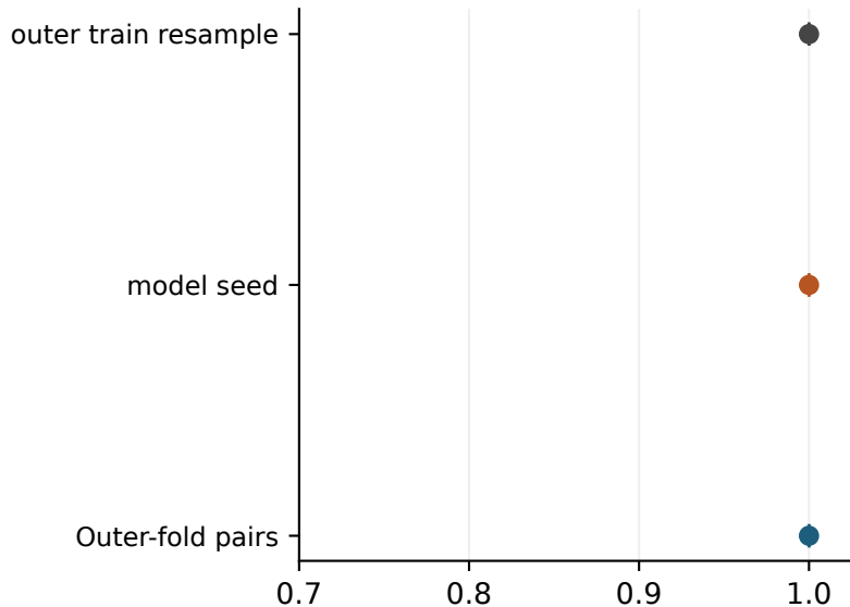
Top-5 Jaccard
