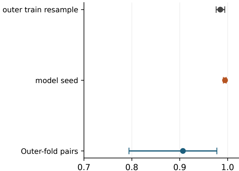
All-feature Spearman
