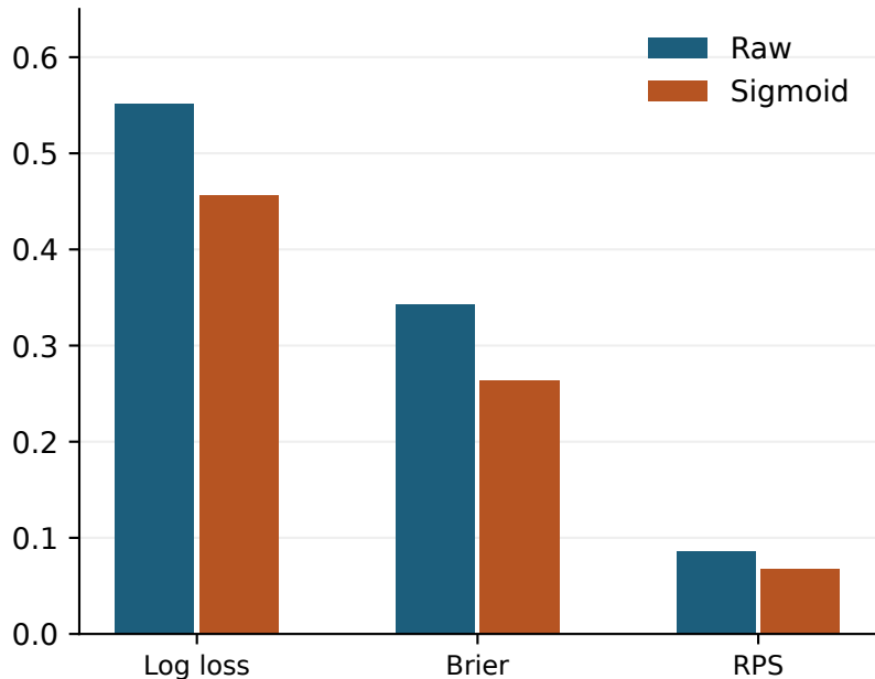
Proper probability scores (lower better)
