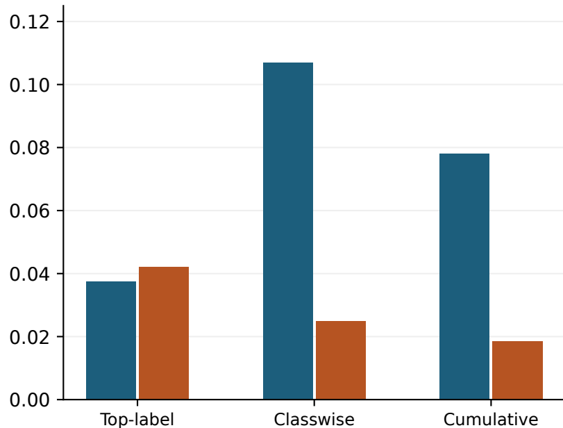
Calibration errors (lower better)
