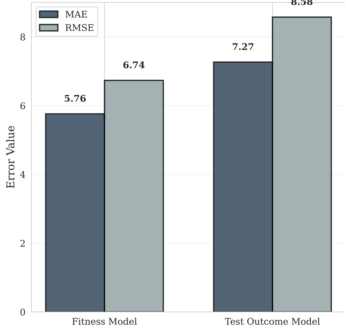
(b) MAE and RMSE Comparison
