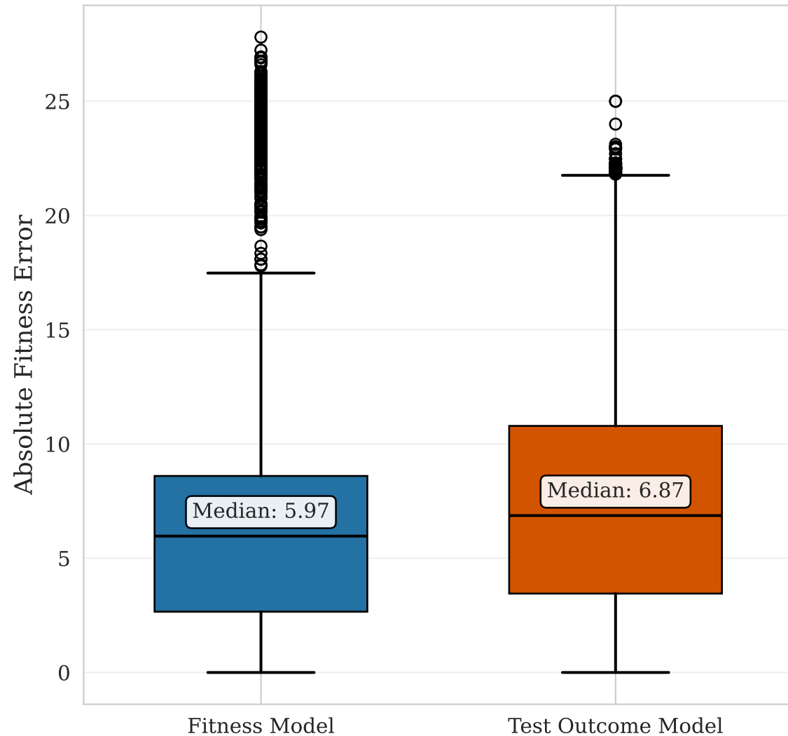
(a) Fitness Prediction Error Distribution
