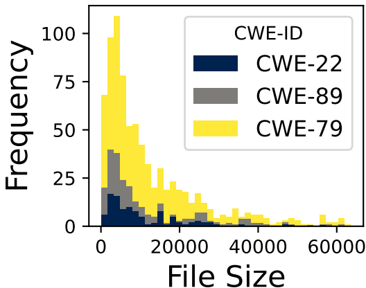
all models
