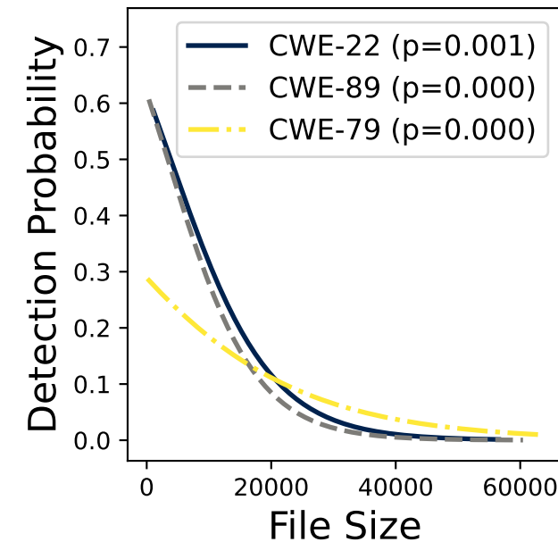
mixtral-8x7b
