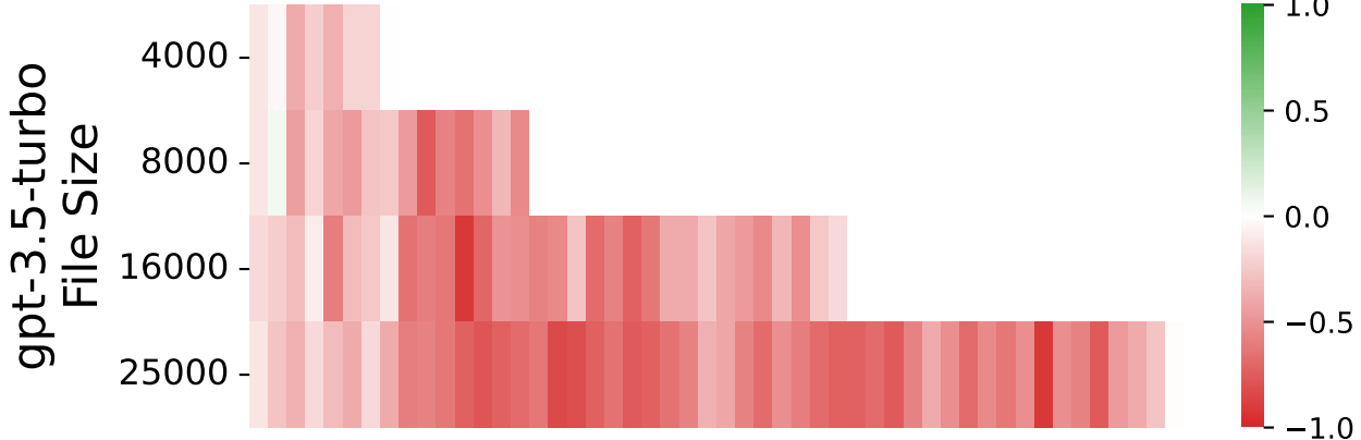
('gpt-3.5-turbo',)
