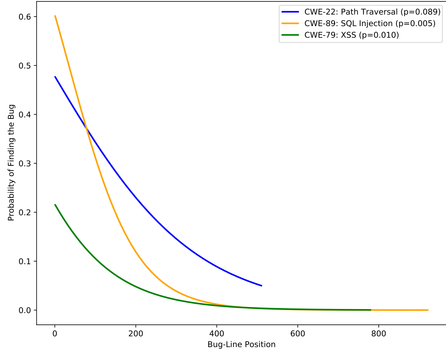
Bug-Line Position vs Probability of Finding the Bug
