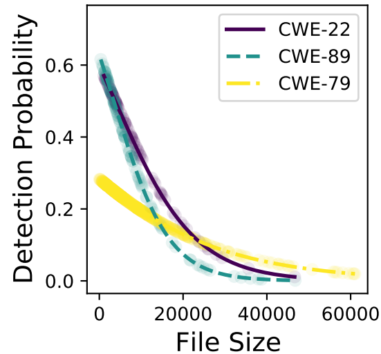
mixtral-8x7b
