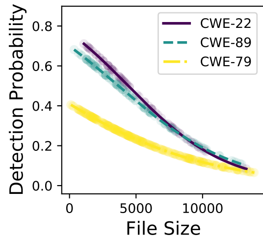
mixtral-8x7b
