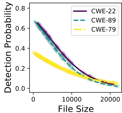
mixtral-8x7b
