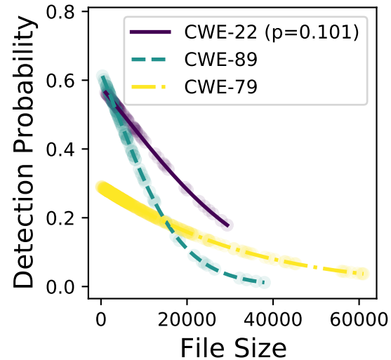
mixtral-8x7b
