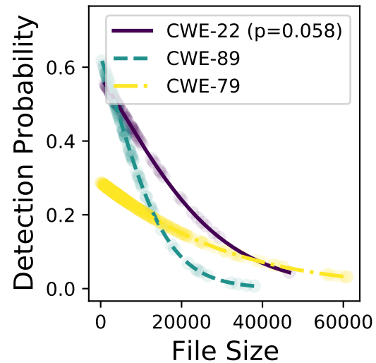
mixtral-8x7b
