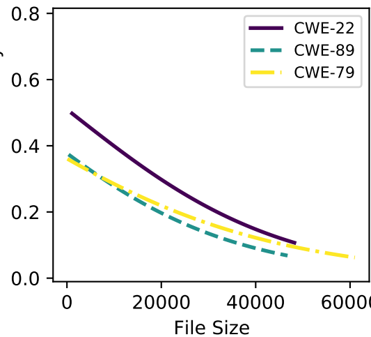
mixtral-8x7b
