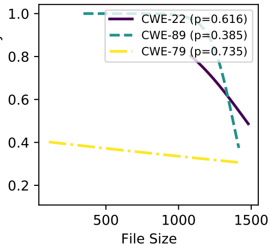
mixtral-8x7b
