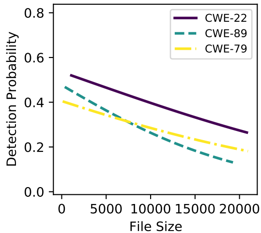
mixtral-8x7b
