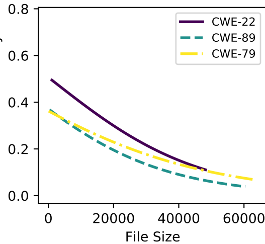
mixtral-8x7b
