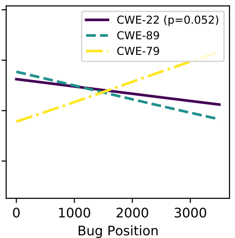
mixtral-8x7b
