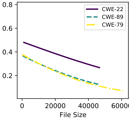
mixtral-8x7b
