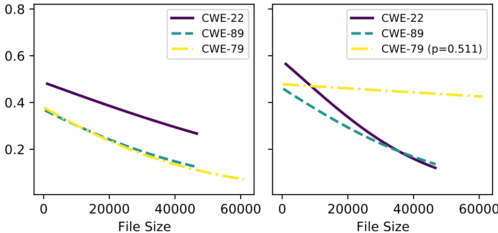
mixtral-8x7b
