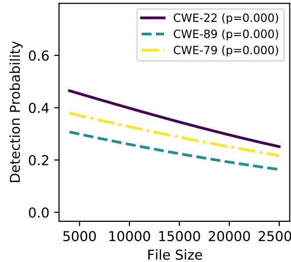
mixtral-8x7b
