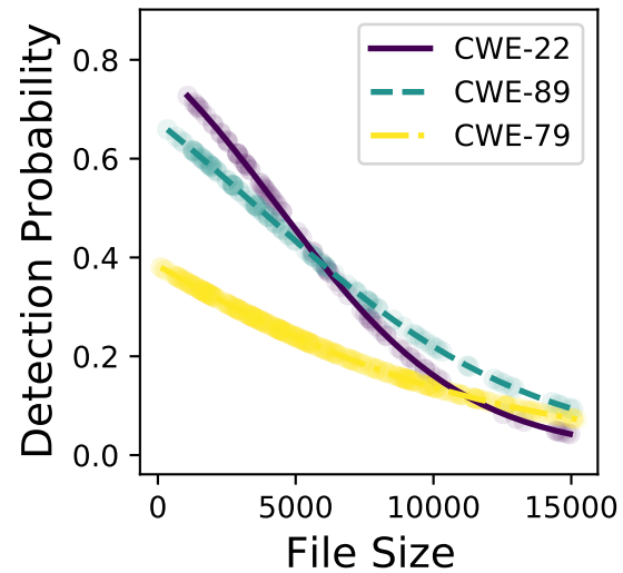
mixtral-8x7b
