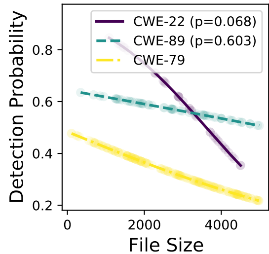
mixtral-8x7b
