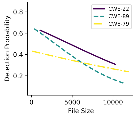
mixtral-8x7b
