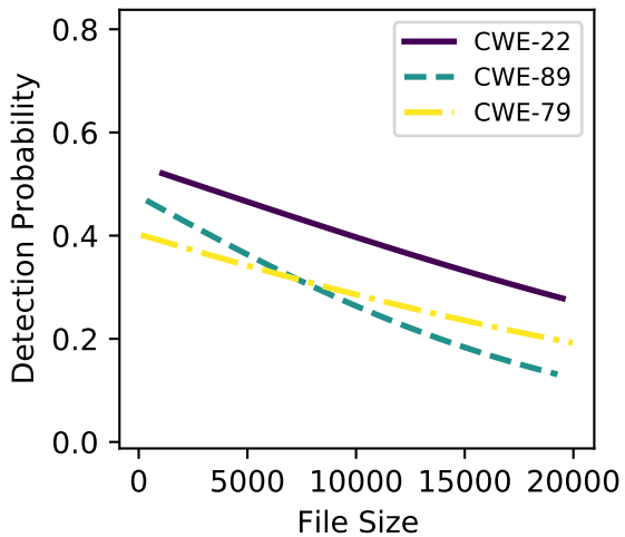
mixtral-8x7b
