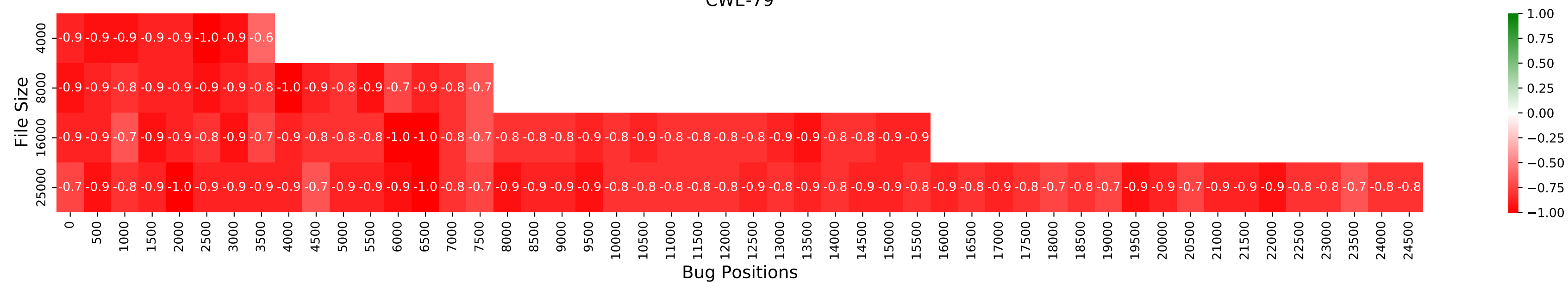
CWE-79
