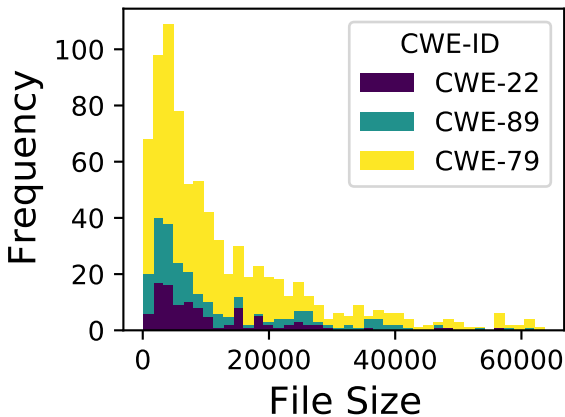
any model
