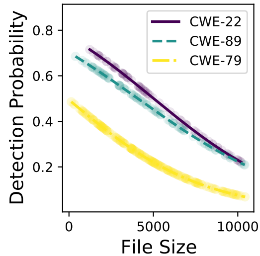
mixtral-8x7b
