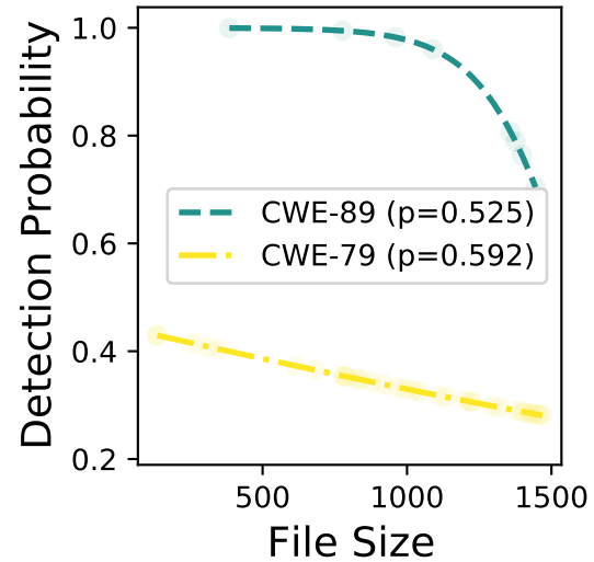
mixtral-8x7b
