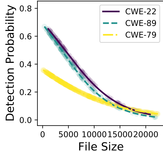
mixtral-8x7b
